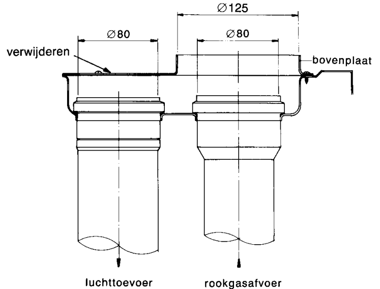
afb. 2 Detail adaptor.
